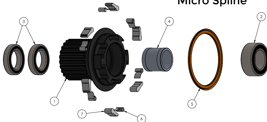
Hydra Mountain Freehub Micro Spline
