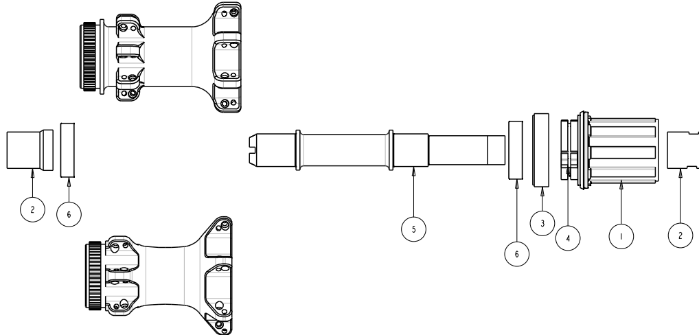
SRX-CL 24H REAR HUB SHELL
